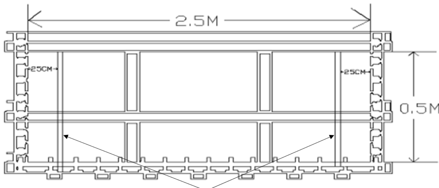
(a) Top view
