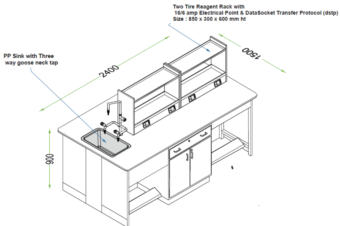
ISLAND TABLE
