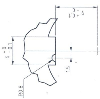
DETAIL C (3:1)
